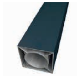
PFOSTEN ALU 90 x 90 mm (RAL7016) Art.1222 L183cm - 86,36 €/St. Art.1225 L200cm - 93,62 €/St.
