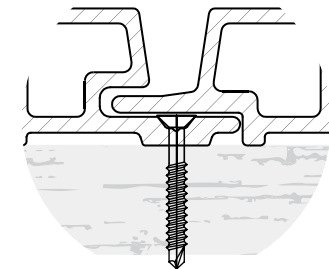
SCREW FASTENING
