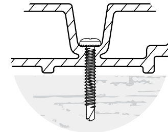
SCREW FASTENING
