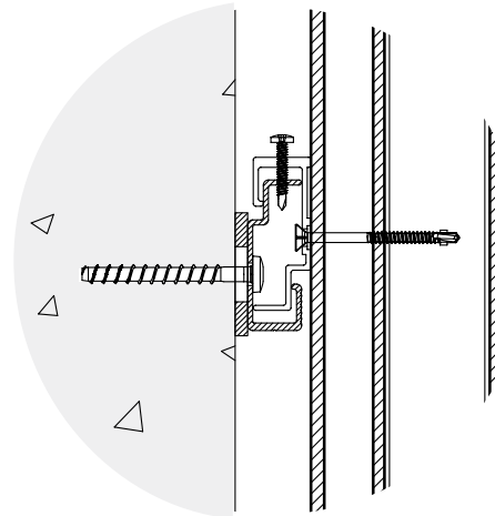
STAPLE FIXING ON CROSSBAR
