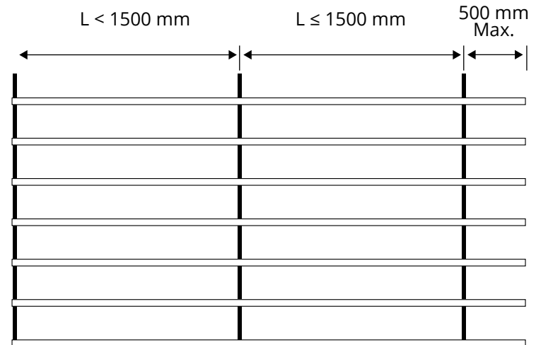
HORIZONTAL INSTALLATION
