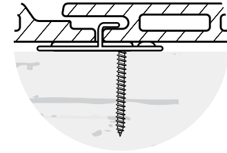
CLIP FASTENING
