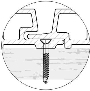
Screw fixing
