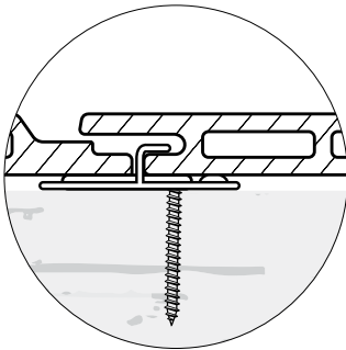
Clip Fixing
