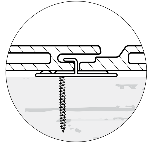
Clip Fixing
