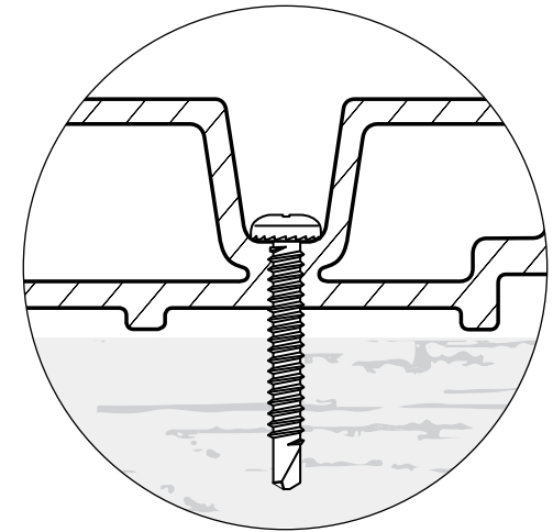
Screw fixing
