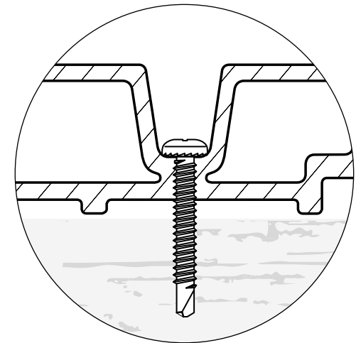
Screw fixing
